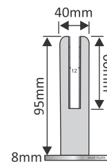
OPTION A : WITH BASE PLATE
